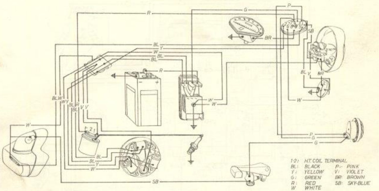
FIG. 37A. WIRING DIAGRAM, VSB 1 WITH BATTERY
