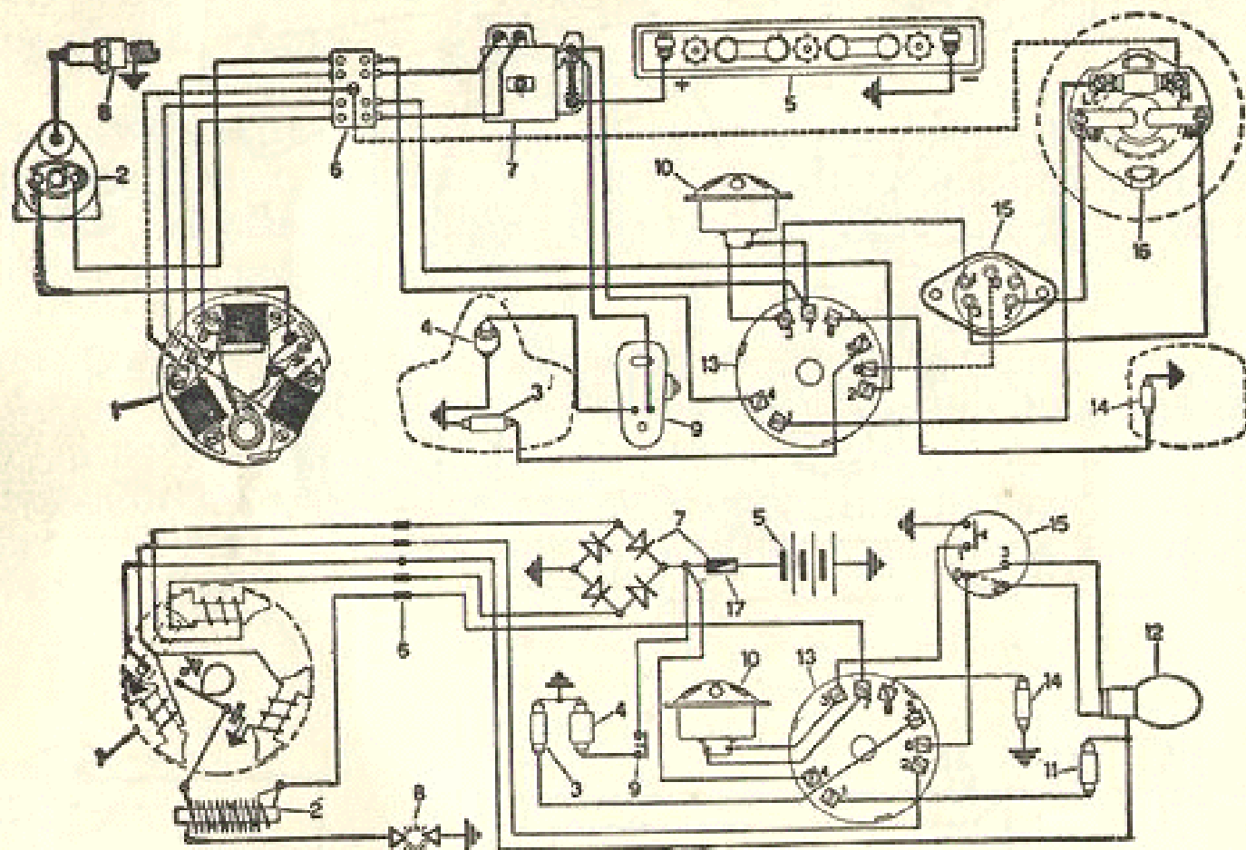
FIG. 35. WIRING DIAGRAM, G.S. VESPA VS 4
